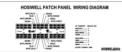
BACK VIEW
